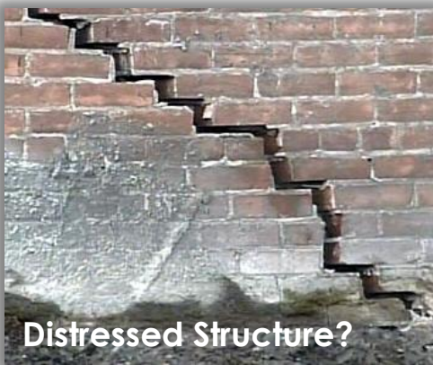
Foundation Underpinning
